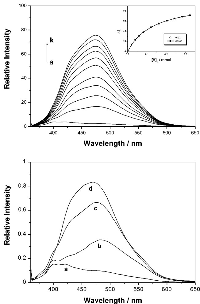
Figure 6. (a) Fluorescence spectral changes of TNS ( 9.4 \times 10^{-6} mol dm -3 ) and the nonlinear least-squares analysis (inset) of the differential intensity ( \Delta I_f ) to calculate the complex stability constant ( K_s ) upon addition of 5 ( 0\text{--}324 \times 10^{-6} mol dm -3 from a to k) in aqueous solution. (b) Fluorescence spectra of TNS ( 9.4 \times 10^{-6} mol dm -3 ) (a) in the absence and in the presence of (b) \beta -cyclodextrin 1 ( 450 \times 10^{-6} mol dm -3 ), (c) bis( \beta -cyclodextrin) 5 ( 20 \times 10^{-6} mol dm -3 ), and (d) metallooligo( \beta -cyclodextrin) 9 ( 20 \times 10^{-6} mol dm -3 ) in aqueous solution.
