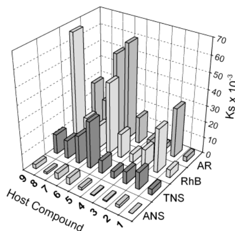
Figure 7. Complex stability constants ( K_s ) for the inclusion complexation of hosts 1–9 with guest molecules in aqueous solution.
