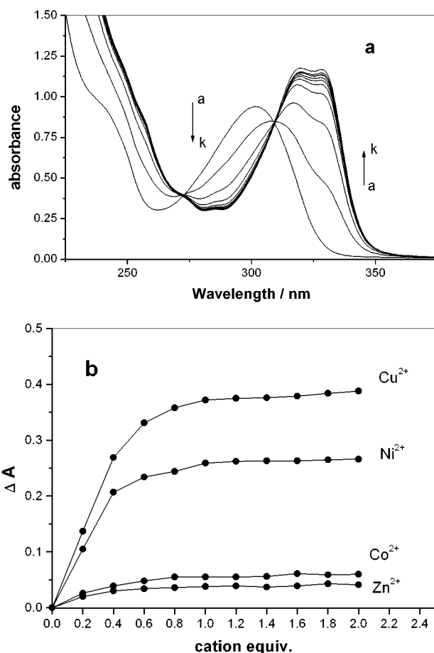
Figure 1. (a) UV-vis spectral change of 2 upon addition of copper(II) ion in aqueous solution. ( [2] = 1.5 \times 10^{-4} mol dm^{-3} , [Cu^{2+}] = 0-3.0 \times 10^{-4} mol dm^{-3} from a to k) (b) spectrophotometric titration of 2 at 302 nm with four metal ions in aqueous solution. ( [2] = 1.5 \times 10^{-4} mol dm^{-3} ; counteranion: NO_3^- ).
