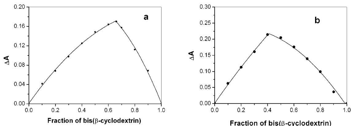
Figure 3. Continuous variation plot of (a) 2 /Cu(II) ( [2] + [\text{Cu}^{2+}] = 1.1 \times 10^{-4} \text{ mol dm}^{-3} ) and (b) 3 /Cu(II) system. ( [3] + [\text{Cu}^{2+}] = 1.5 \times 10^{-4} \text{ mol dm}^{-3} ).
