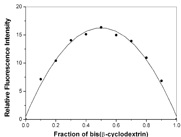
Figure 5. Continuous variation plot of 6 /AR system. ( [\text{bis}(\beta\text{-cyclodextrin}) \text{ unit}] + [\text{AR}] = 1.0 \times 10^{-5} \text{ mol dm}^{-3} ).
