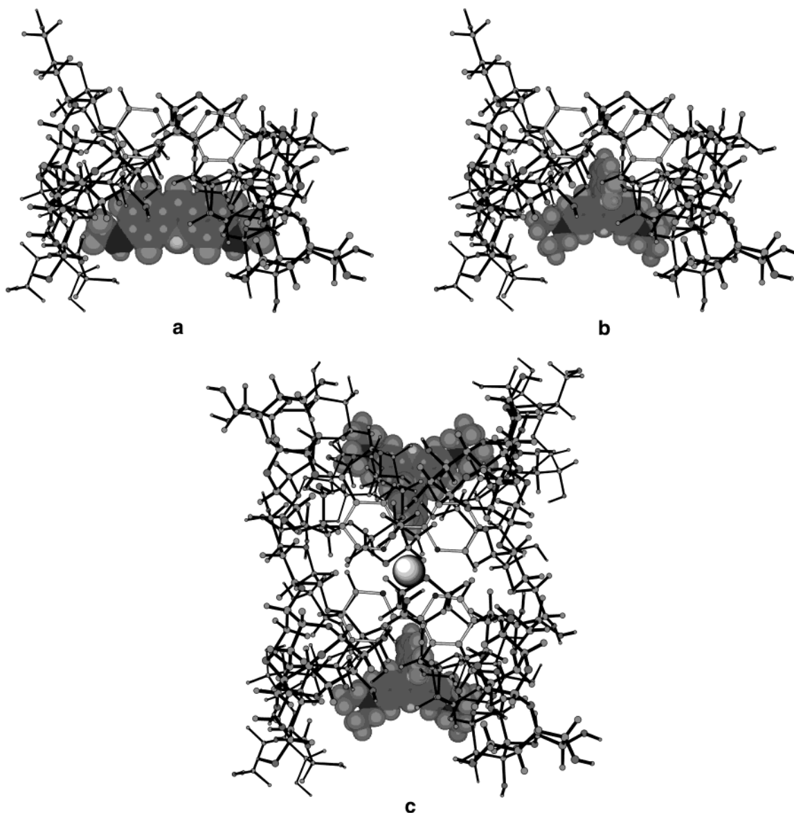
Figure 8. Inclusion complexation modes of guest molecule with bis( \beta -cyclodextrin) and metallooligo( \beta -cyclodextrin); model system: (a) host 2 + AR, (b) host 2 + RhB, (c) host 6 + RhB.
