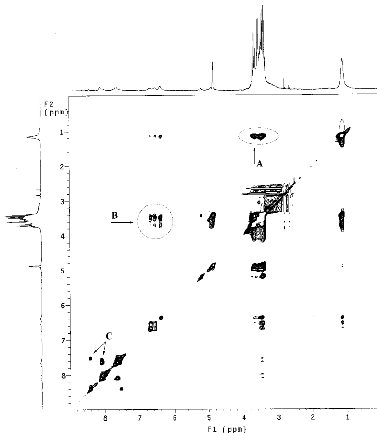
Figure 10. ^1\text{H} NOESY spectrum (300 MHz) of a mixture of 2 -Ni(II) with RhB ( [\text{2-Ni(II)}] = [\text{RhB}] = 5.0 \times 10^{-4} \text{ mol dm}^{-3} ) in \text{D}_2\text{O} at 298 K with a mixing time of 800 ms.
