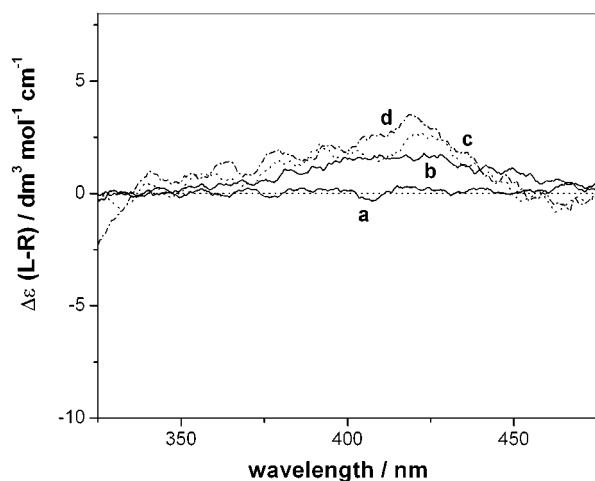
Figure 9. Circular dichroism spectra of methyl orange ( 10.7 \times 10^{-6} \text{ mol dm}^{-3} ) (a) without and (b) with \beta -cyclodextrin ( 1600 \times 10^{-6} \text{ mol dm}^{-3} ), (c) with bis( \beta -cyclodextrin) 2 ( 50.6 \times 10^{-6} \text{ mol dm}^{-3} ), and d) with metallooligo( \beta -cyclodextrin) 6 ( 48 \times 10^{-6} \text{ mol dm}^{-3} ).
