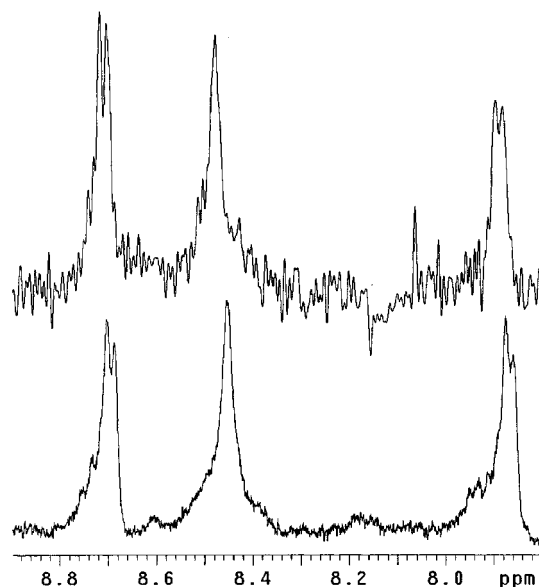
Figure 2. Partial ^1\text{H} NMR spectra (300 MHz, \text{D}_2\text{O} ) of bis( \beta -cyclodextrin) 2 (the lower) and 2 -Ni(II) complex (the upper).
