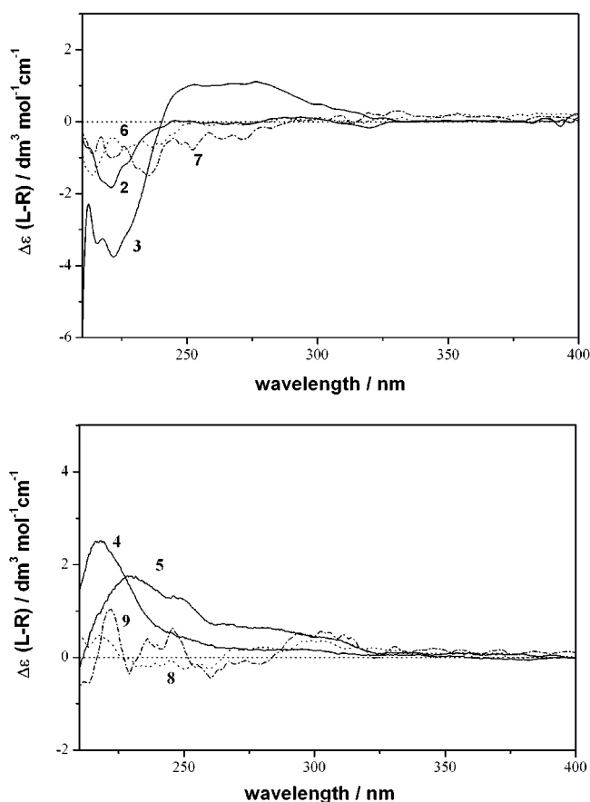
Figure 4. Circular dichroism spectra of hosts 2–9 ( 1 \times 10^{-4} \text{ mol dm}^{-3} ) in aqueous solution at 25 °C.
